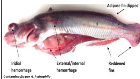
FIGURE 21c Aeromonas
