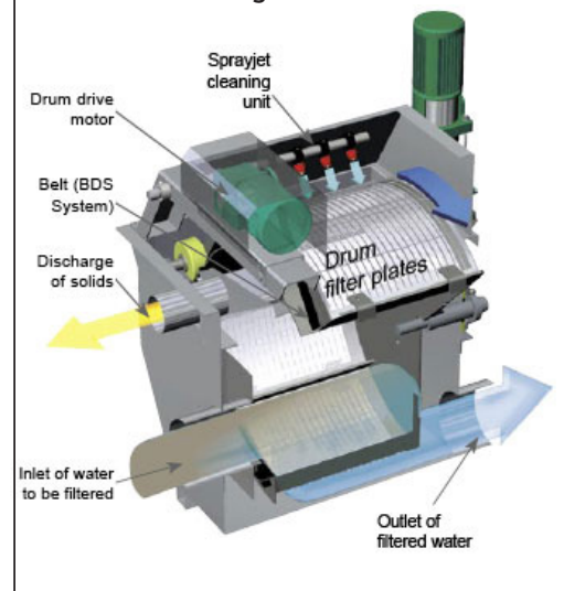
FIGURE 5a Rotating drum filter
